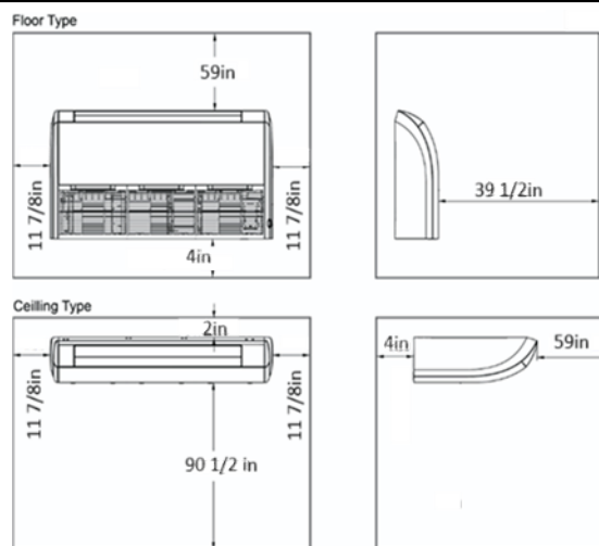
Minimum indoor unit clearances
